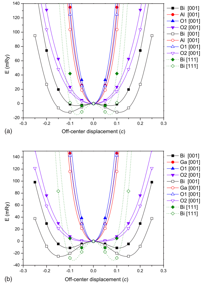
FIG. 4. (Color online) Profiles of PES for the displacement of ions along the tetragonal [001] (lines) and rhombohedral [111] (dot lines) in cubic \text{BiAlO}_3 (up) and \text{BiGaO}_3 (down) at predicted equilibrium lattice constant and 1% volume expansion indicated by solid and vacuity symbols, respectively.
